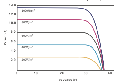
I-V CURVES OF PV MODULE (385W)
